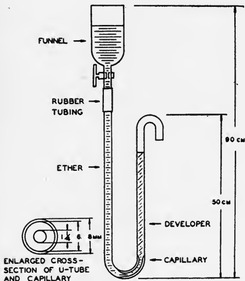
FIG. 1. U-tube extractor.
